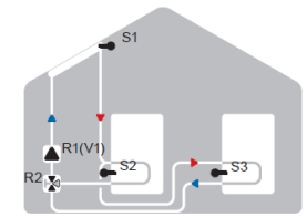
Solar with 2 hot water storage tanks and 3-way valve
